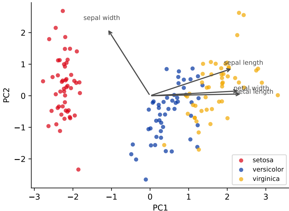
iris biplot: samples + feature loadings
