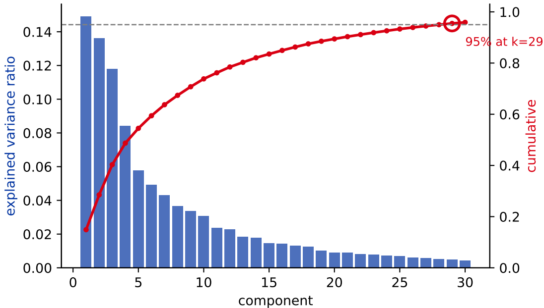
scree + cumulative explained variance (digits)
