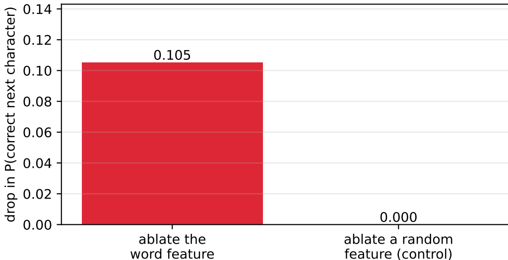
deleting one feature while the RNN spells "iixxz"
