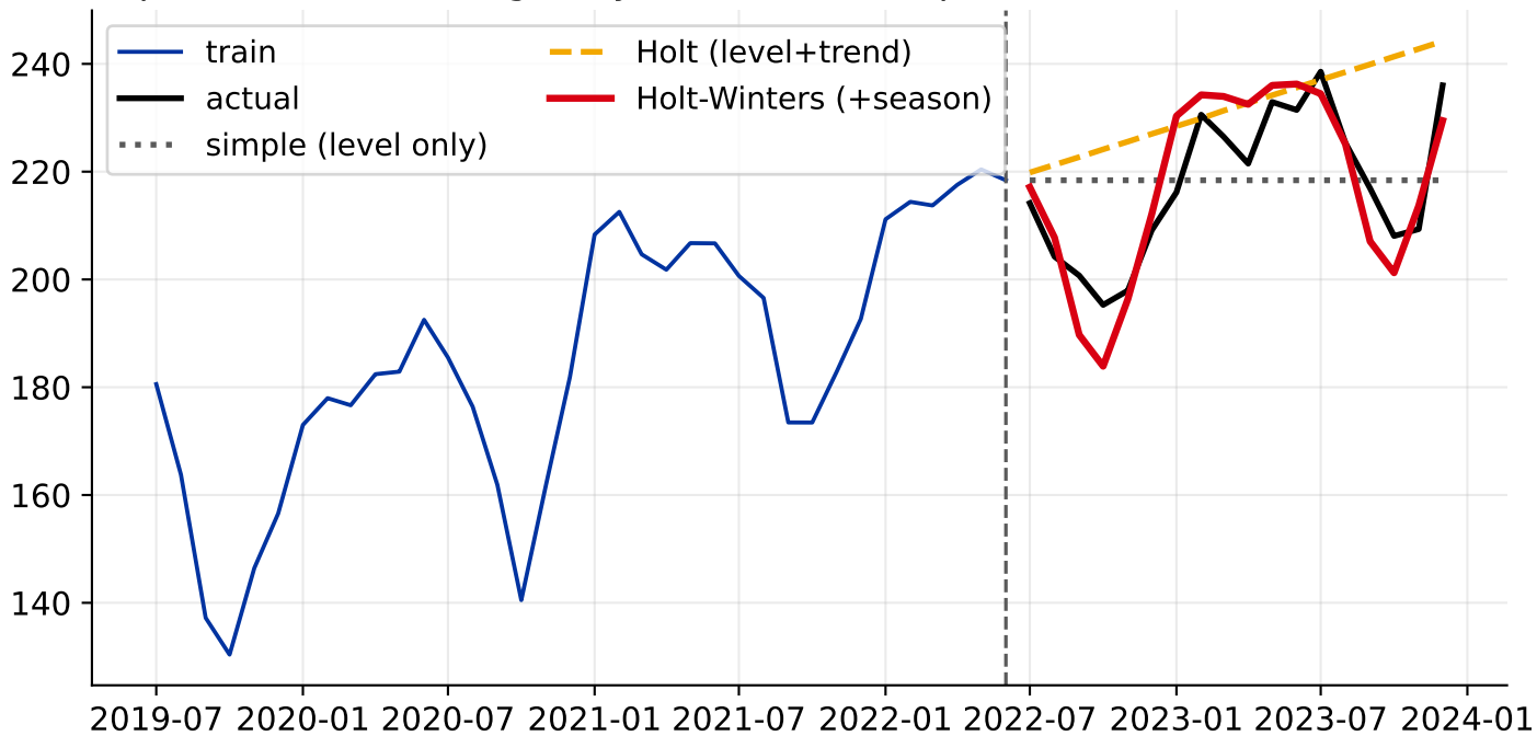
Exponential smoothing: only Holt-Winters captures the season
