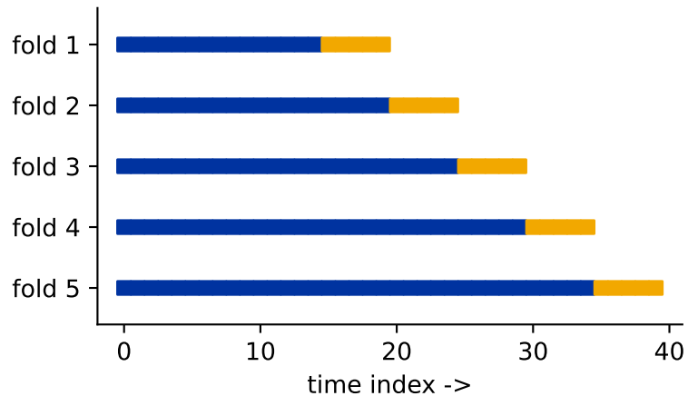
expanding window (the default)
