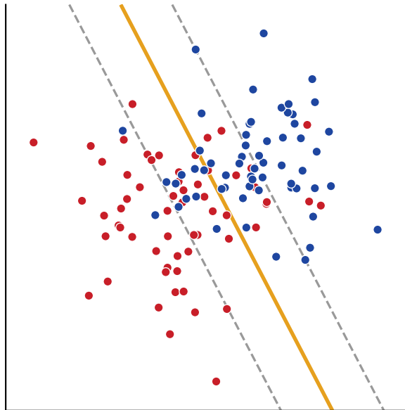
C = 100 (narrow margin, 58 SVs)
