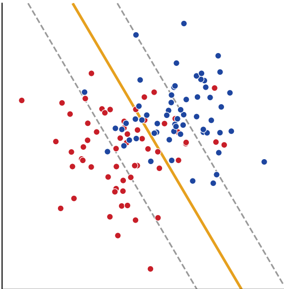
C = 0.05 (wide margin, 66 SVs)
