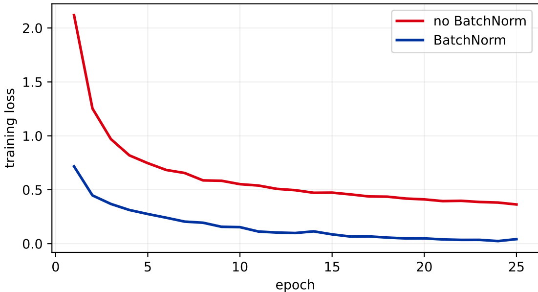
BatchNorm speeds up and stabilizes training
