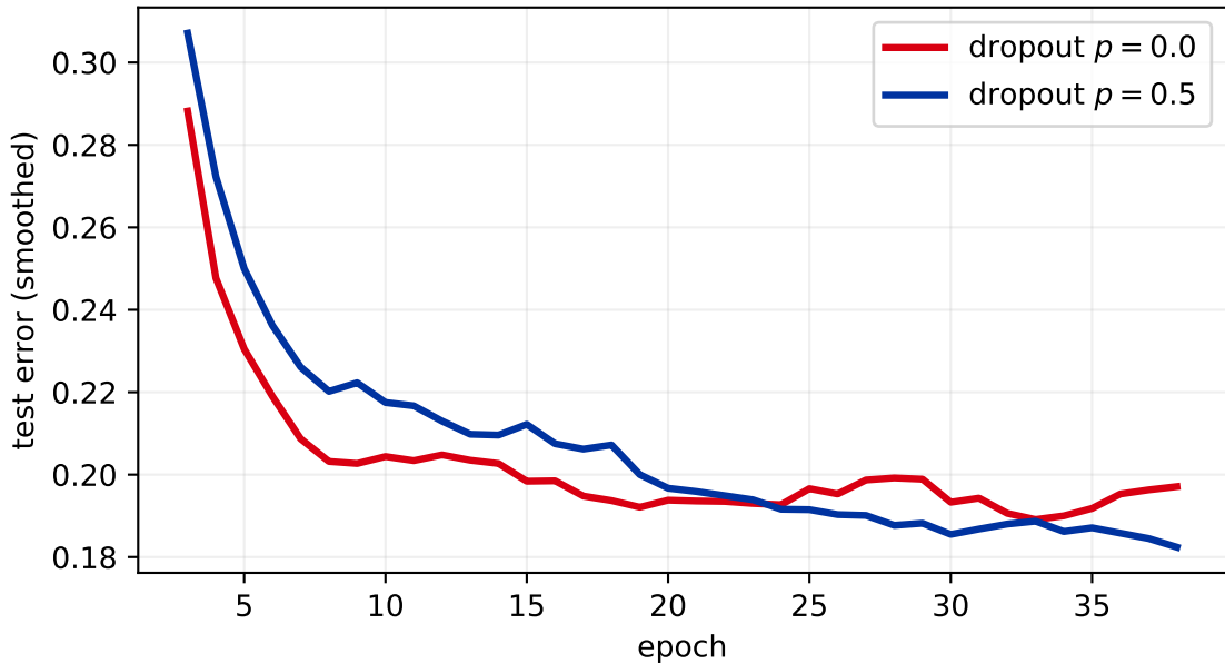
Dropout curbs overfitting (Fashion-MNIST, 1.5k train)
