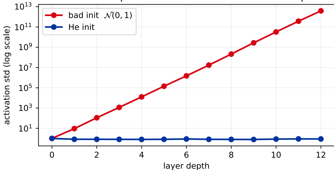
Good init keeps the activation scale stable with depth
