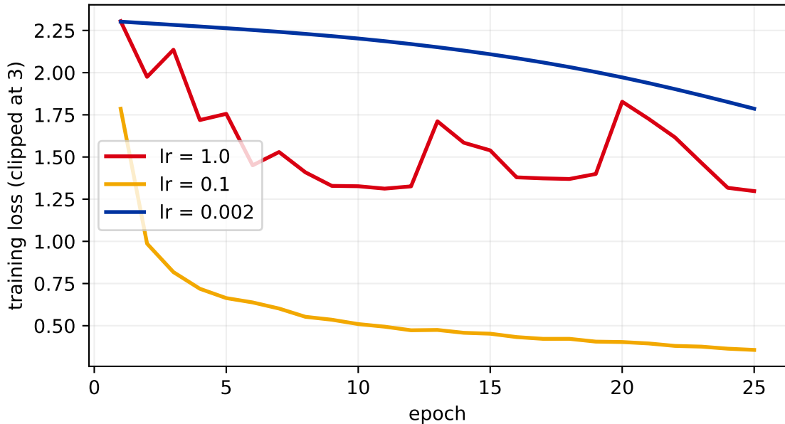
Learning rate: too high diverges, too low crawls
