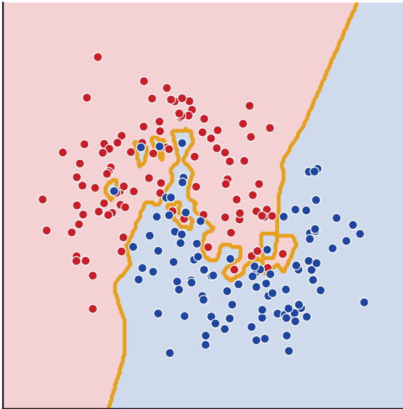
k = 1 (jagged, overfit)
