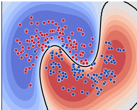
SVM (RBF) proba: soft
