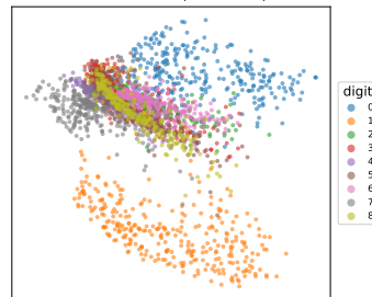
Autoencoder (nonlinear)
