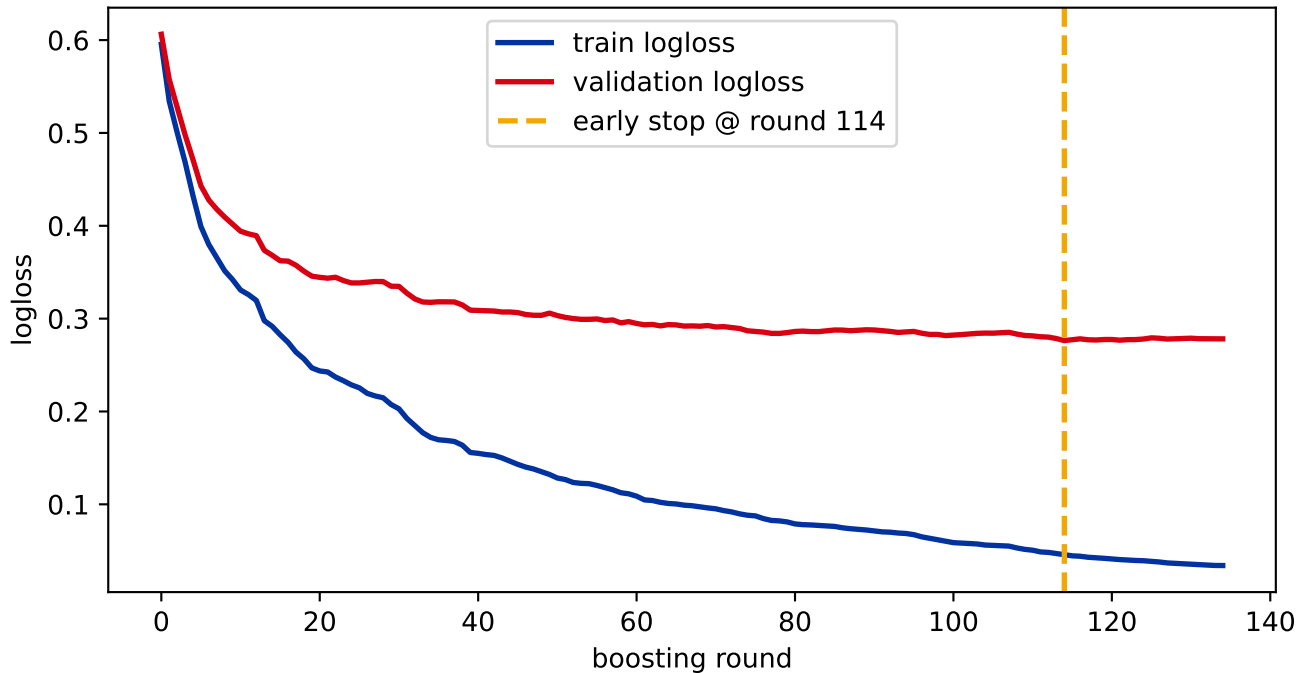
Early stopping: validation logloss stops improving
