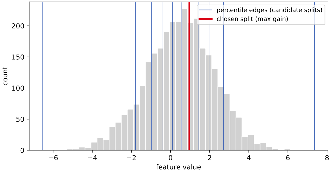
Approximate split finding: candidates = percentile bin edges
