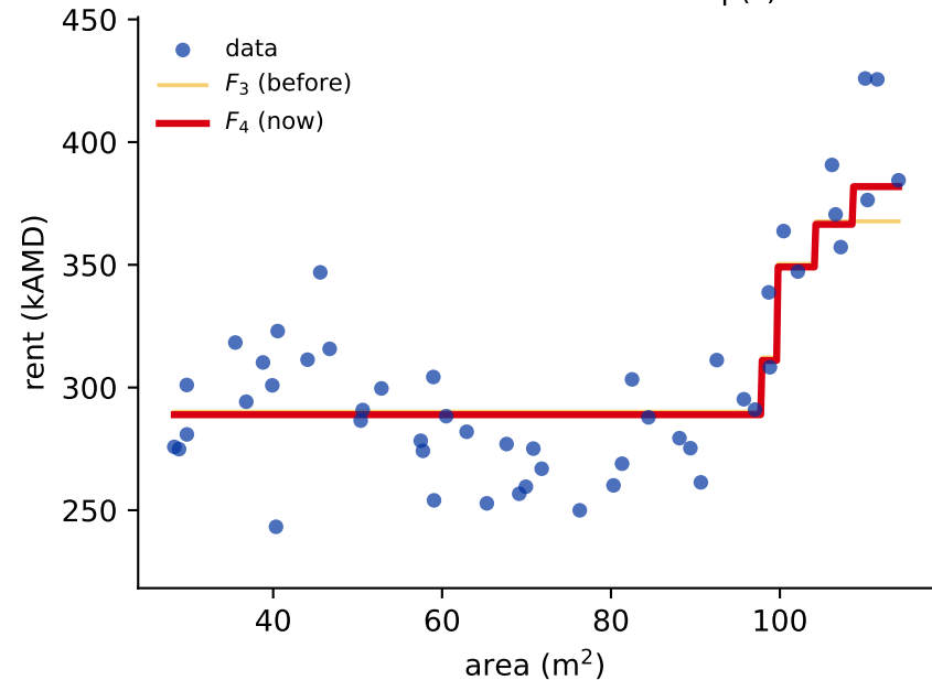
round 4: ensemble of 4 stump(s)
