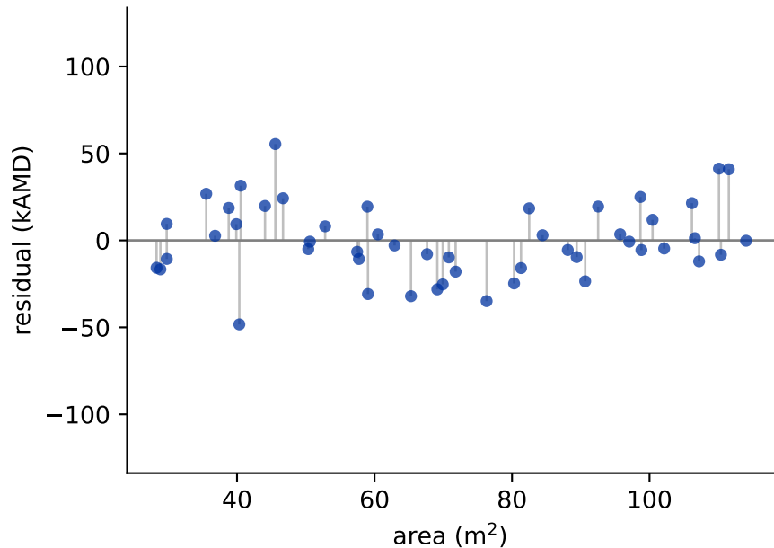
what's left: residuals r_6 = y - F_6
