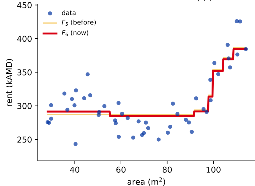
round 6: ensemble of 6 stump(s)
