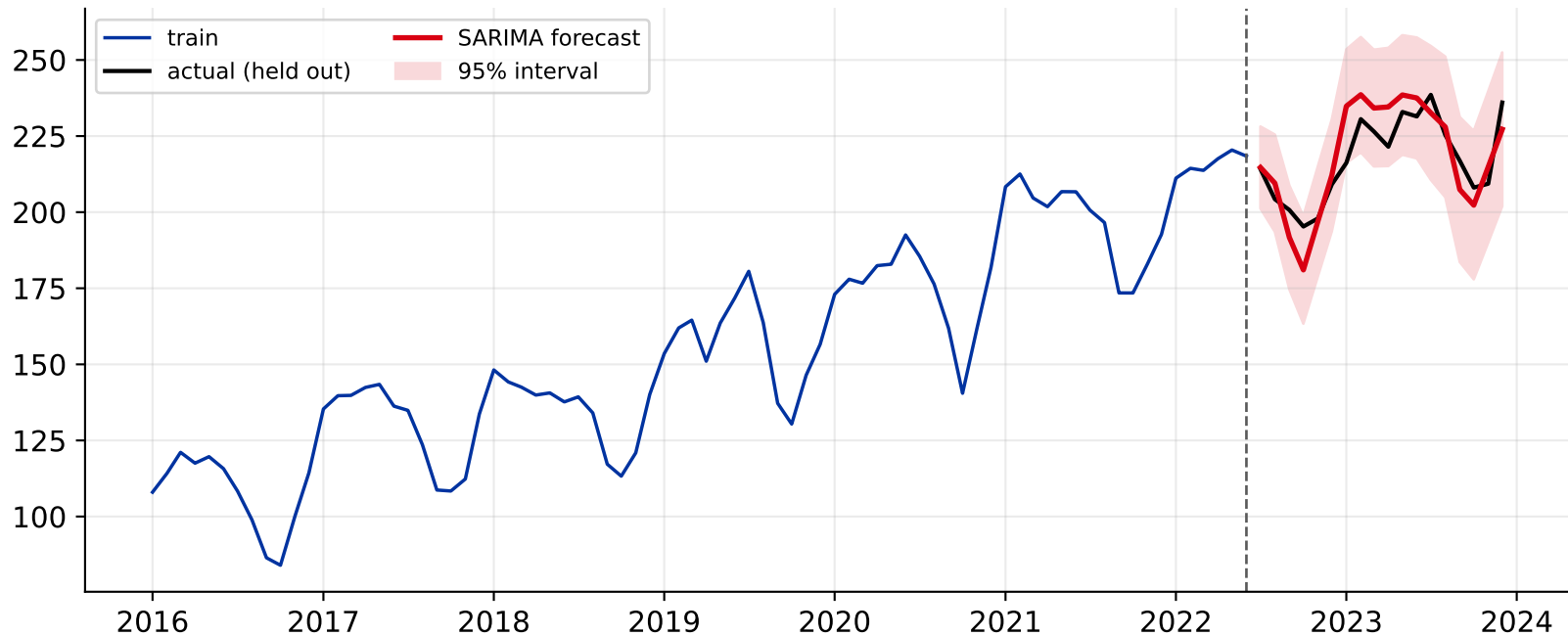
SARIMA(1,1,1)(1,1,0) 12 forecast
