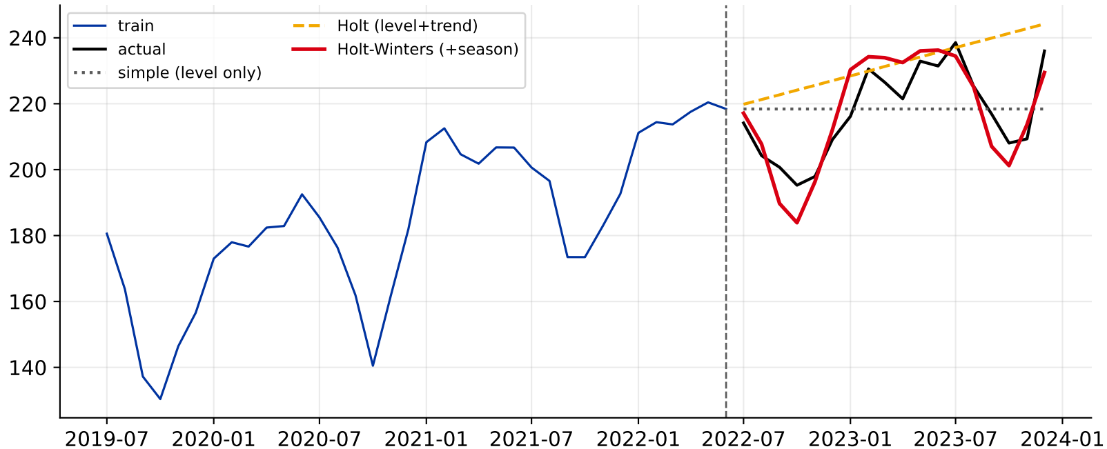
Exponential smoothing: only Holt-Winters captures the season
