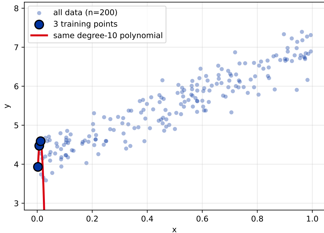
Same polynomial on all 200 points wildly wrong everywhere else (huge test error)
