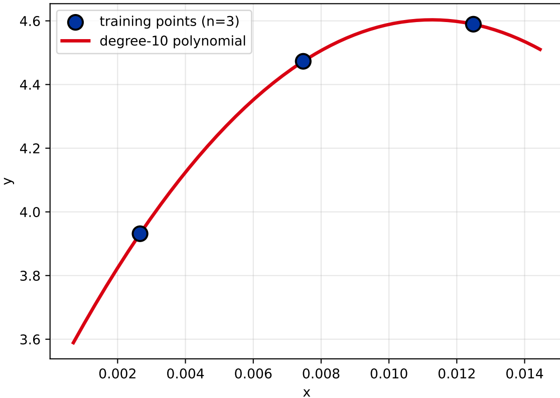
Zoomed in: degree-10 polynomial fits 3 training points perfectly (train MSE = 0)
