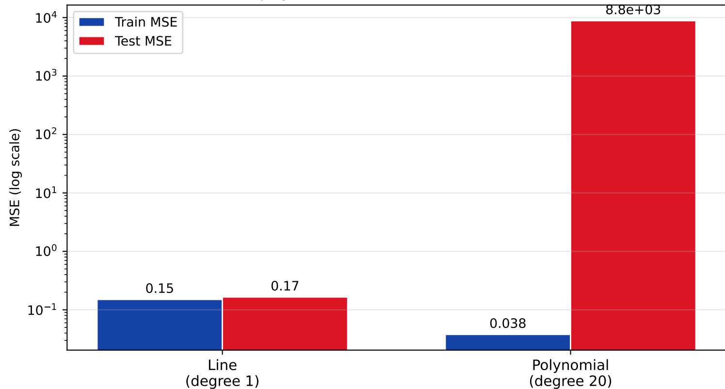
Train vs test MSE: line versus high-degree polynomial the polynomial wins on train and loses on test
