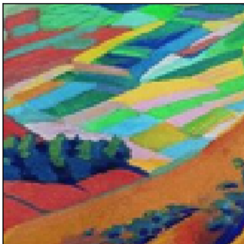
original (zoomed)
