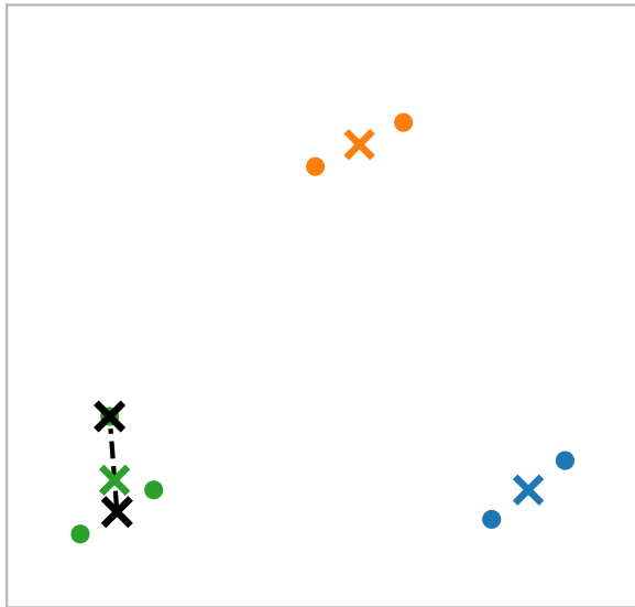
merge 4: cheapest merge, d = 0.75
