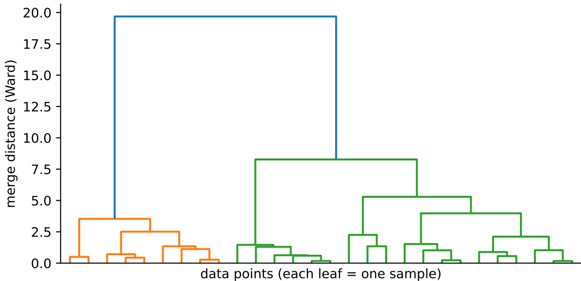
Dendrogram: cut the tree to choose #clusters
