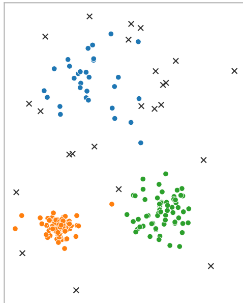
HDBSCAN \rightarrow 3 clusters (adapts to each density)
