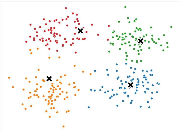
k-means --- iteration 3
