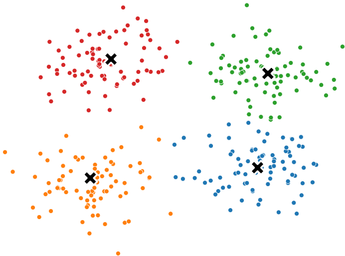
k-means --- iteration 4
