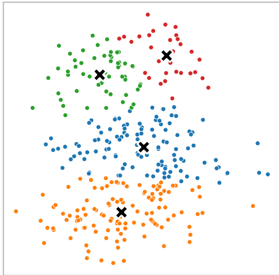
one bad random init inertia = 1055
