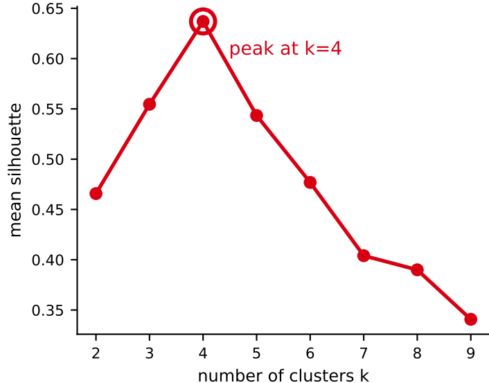
silhouette: has a real maximum - argmax it
