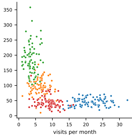
k-means after standardizing
