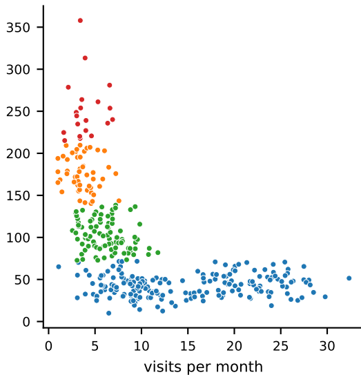
k-means on raw numbers
