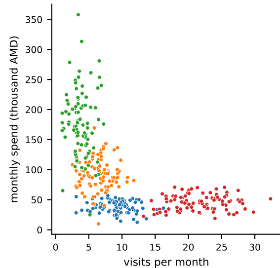
the truth: four segments
