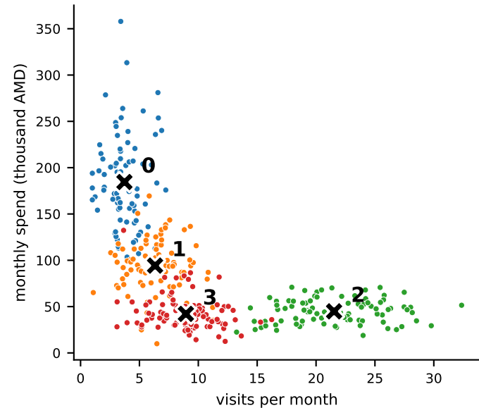
the clustering (X = centroid)
