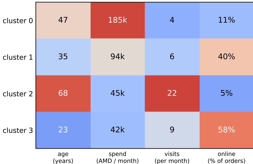
centroid profile (color = z-score, text = actual value)
