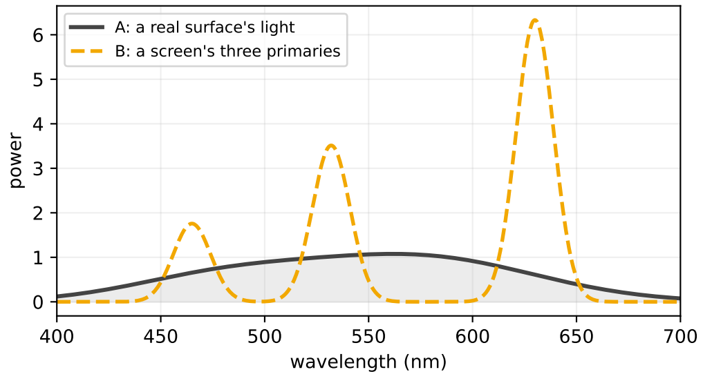
Different light, identical cone responses (this is why a screen only needs three primaries)
