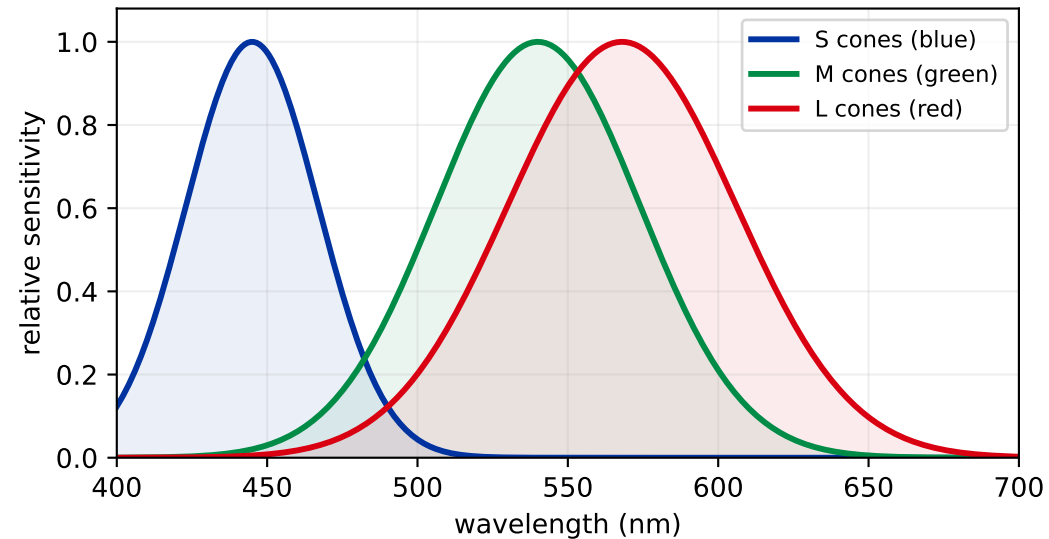
Three cone types -> three numbers per point
