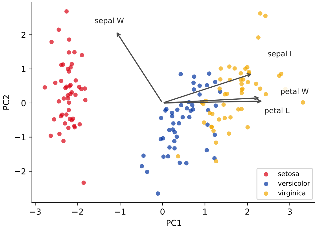
iris biplot: samples + feature loadings
