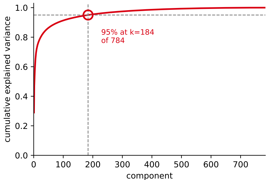
cumulative: the tail is long and flat
