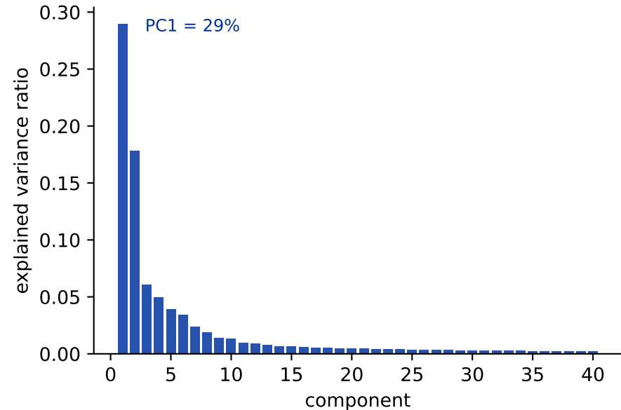
scree: the first 40 components
