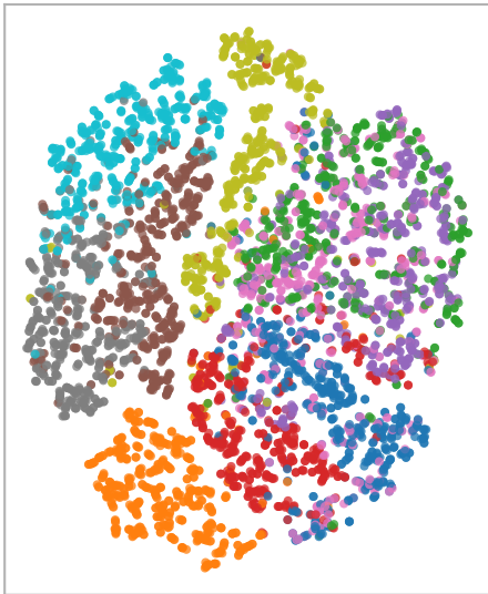
perplexity = 5
