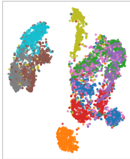
perplexity = 100
