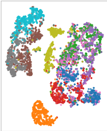
perplexity = 30
