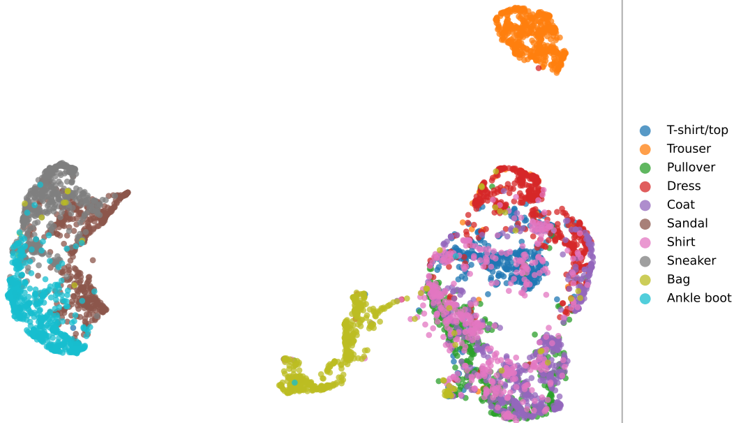
UMAP of Fashion-MNIST (5000 items)
