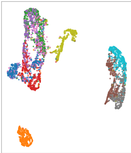
random_state = 42
