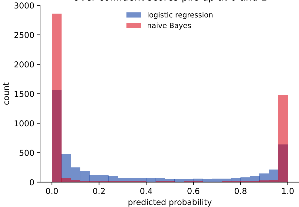
Over-confident scores pile up at 0 and 1
