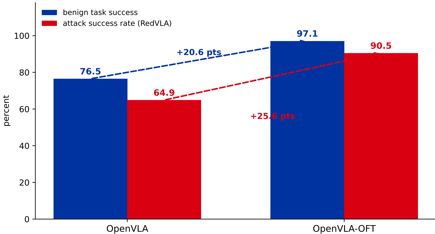
OpenVLA vs OpenVLA-OFT under RedVLA evaluation
