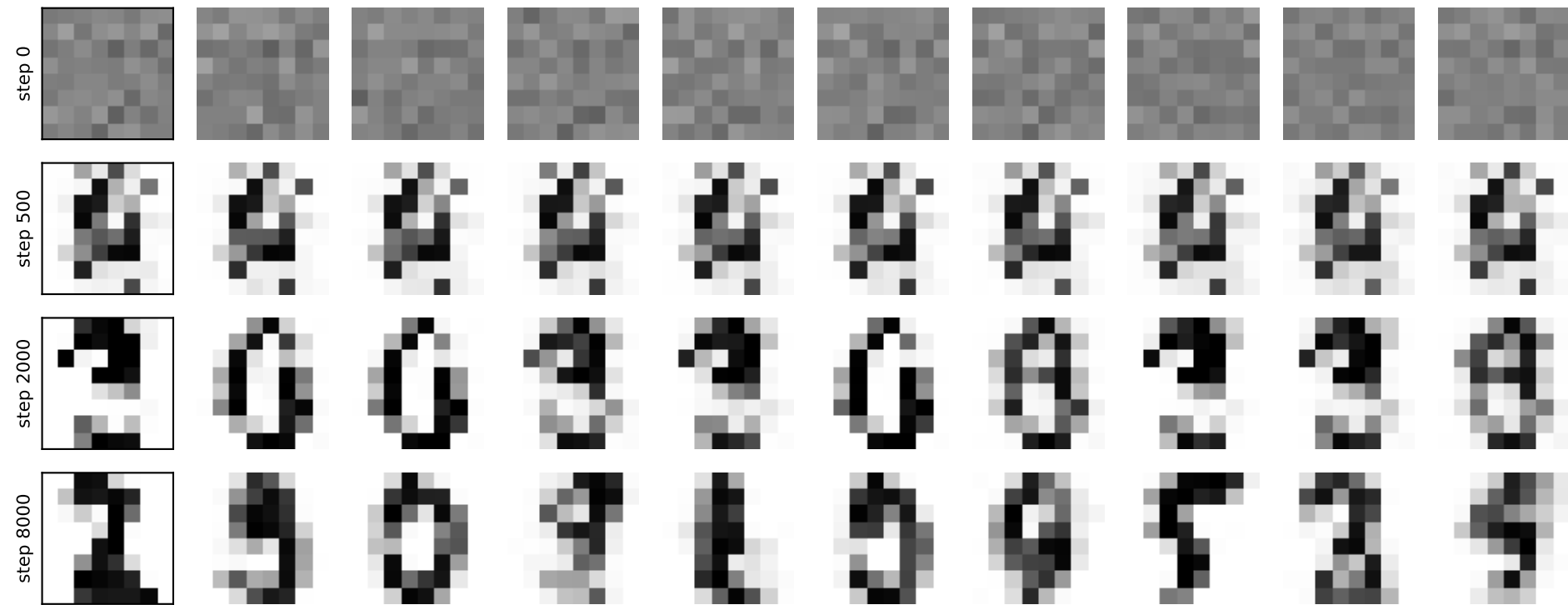
Same 10 latent vectors, followed through training
