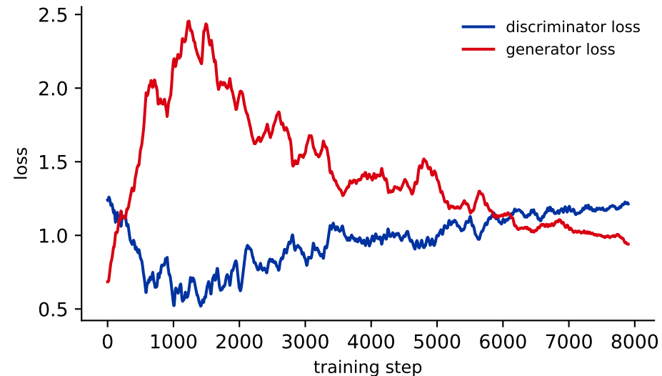
Neither loss is going anywhere
