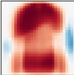
PC1 (29%)
