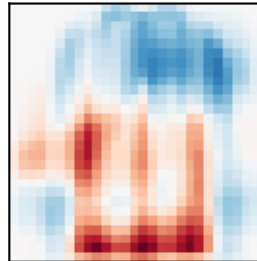
PC5 (4%)
