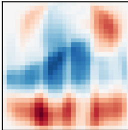
PC4 (5%)
