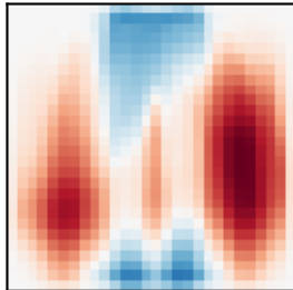
PC2 (18%)
