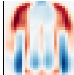
PC6 (3%)
