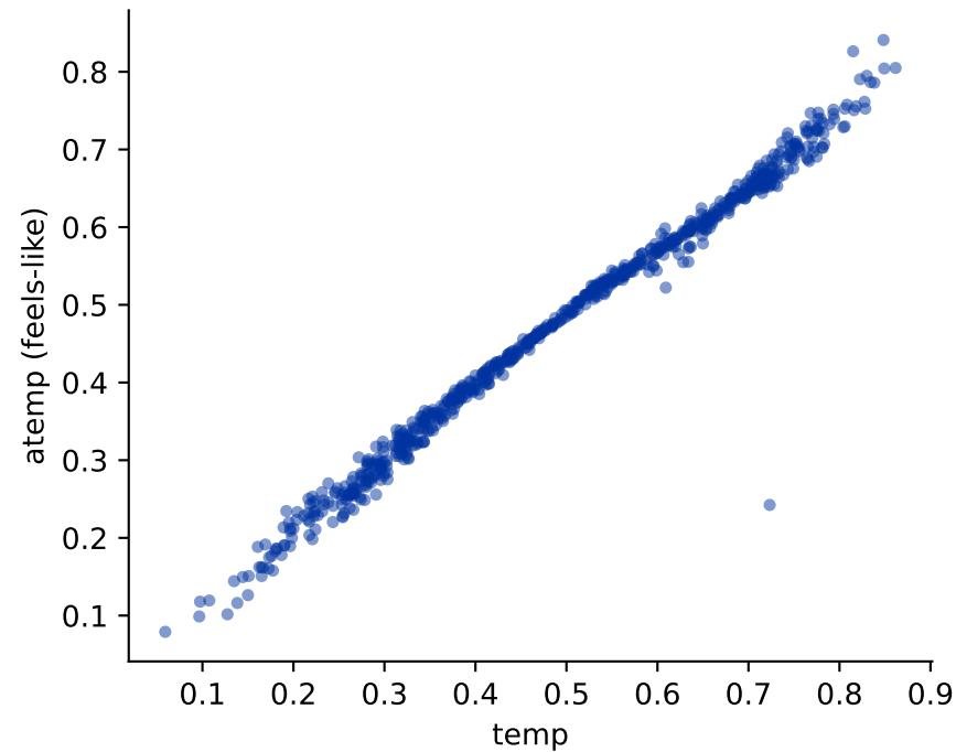
real data: temp \approx atemp (correlated)
