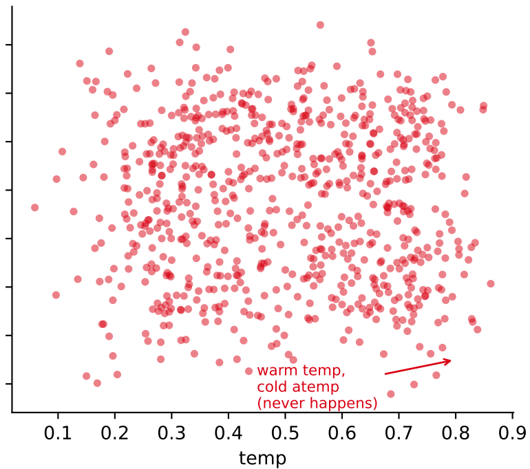
after permuting temp: impossible rows
