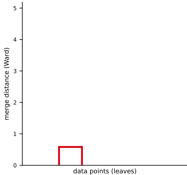
dendrogram
