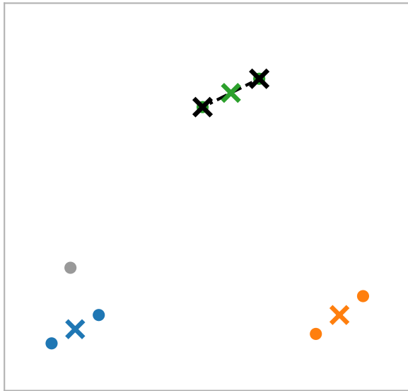
merge 3: cheapest merge, d = 0.67
