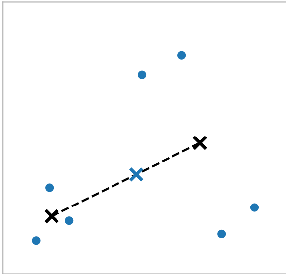
merge 6: cheapest merge, d = 4.63
