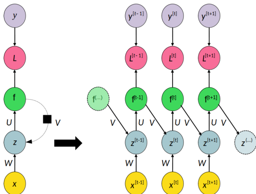
Figure: RNN with feedback connection from the output to the hidden layer. The RNN is only allowed to send f to future time points and, hence, z^{[t-1]} is connected to z^{[t]} only indirectly, via the predictions f^{[t-1]} .
