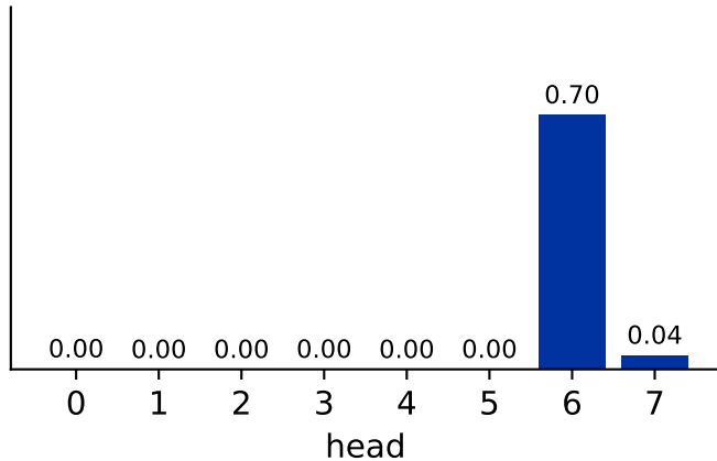
layer 1: induction pattern
