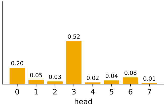
layer 0: attends to the previous token
