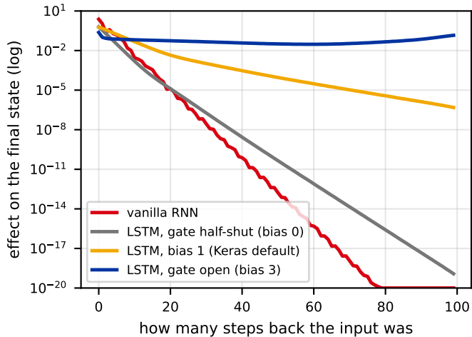
Before training: how far back does the net 'hear'?
