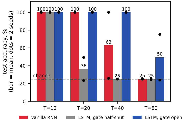
After training: recall the first token after T steps
