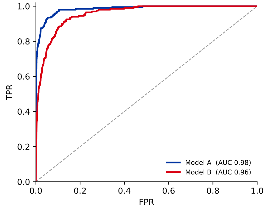
ROC: ``both look great''
