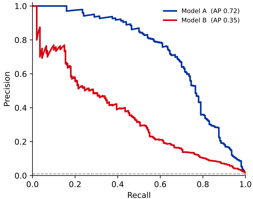
PR: Model B collapses
